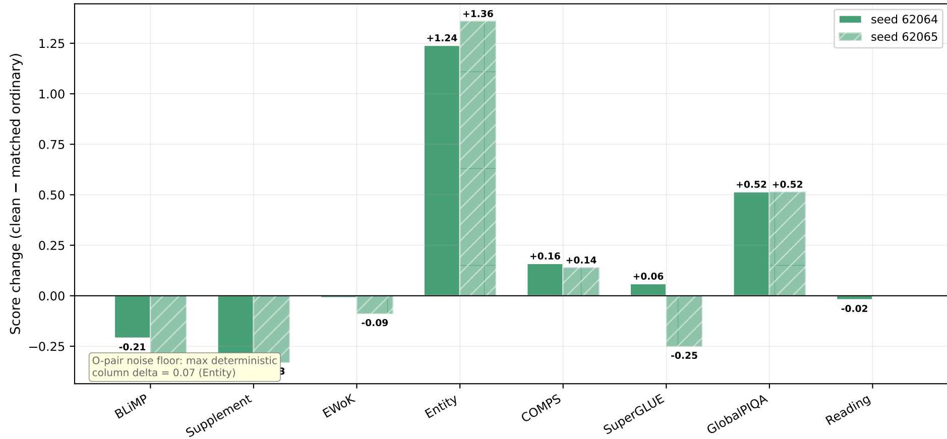
Per-Component Gains and Costs: Principle-Guided v5 vs Matched Ordinary Continuation
