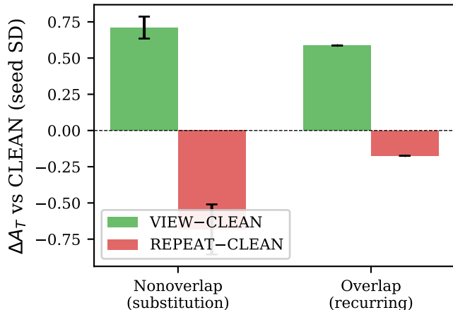
(b) Designed compact (seed43022; bars = 3-seed SD)
