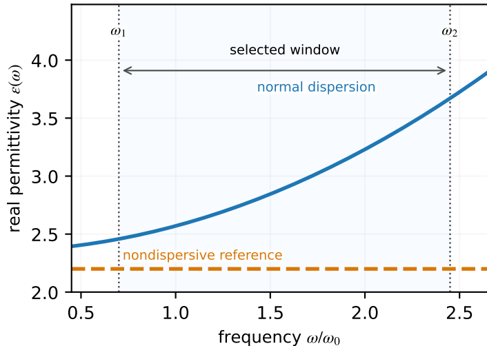
Permittivity model
