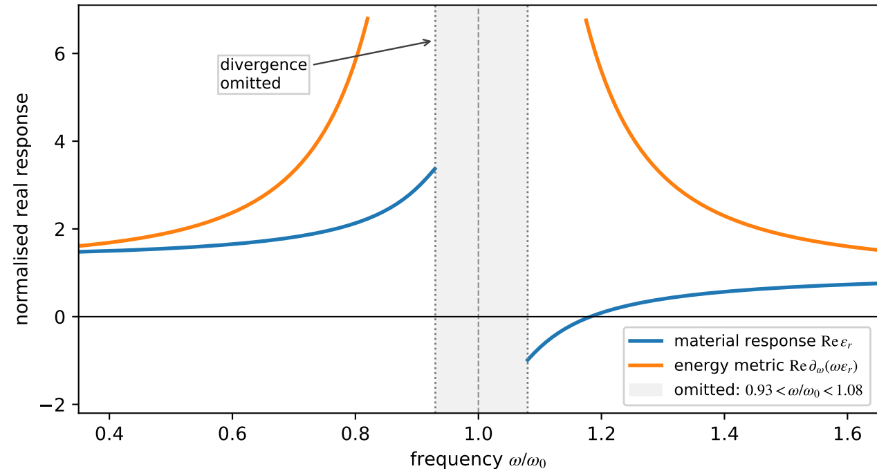
Lorentz response and stored-energy metric
