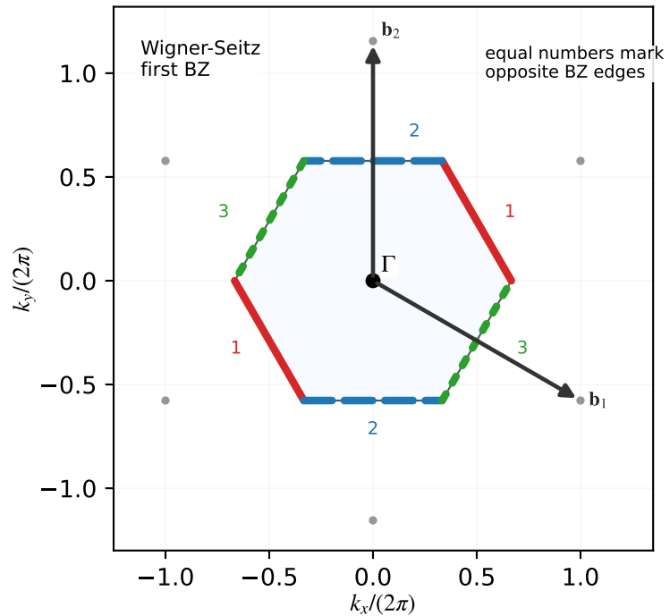
First BZ and reciprocal vectors
