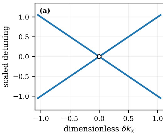
Linear crossing
