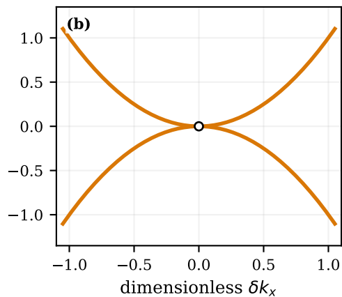
Quadratic touching
