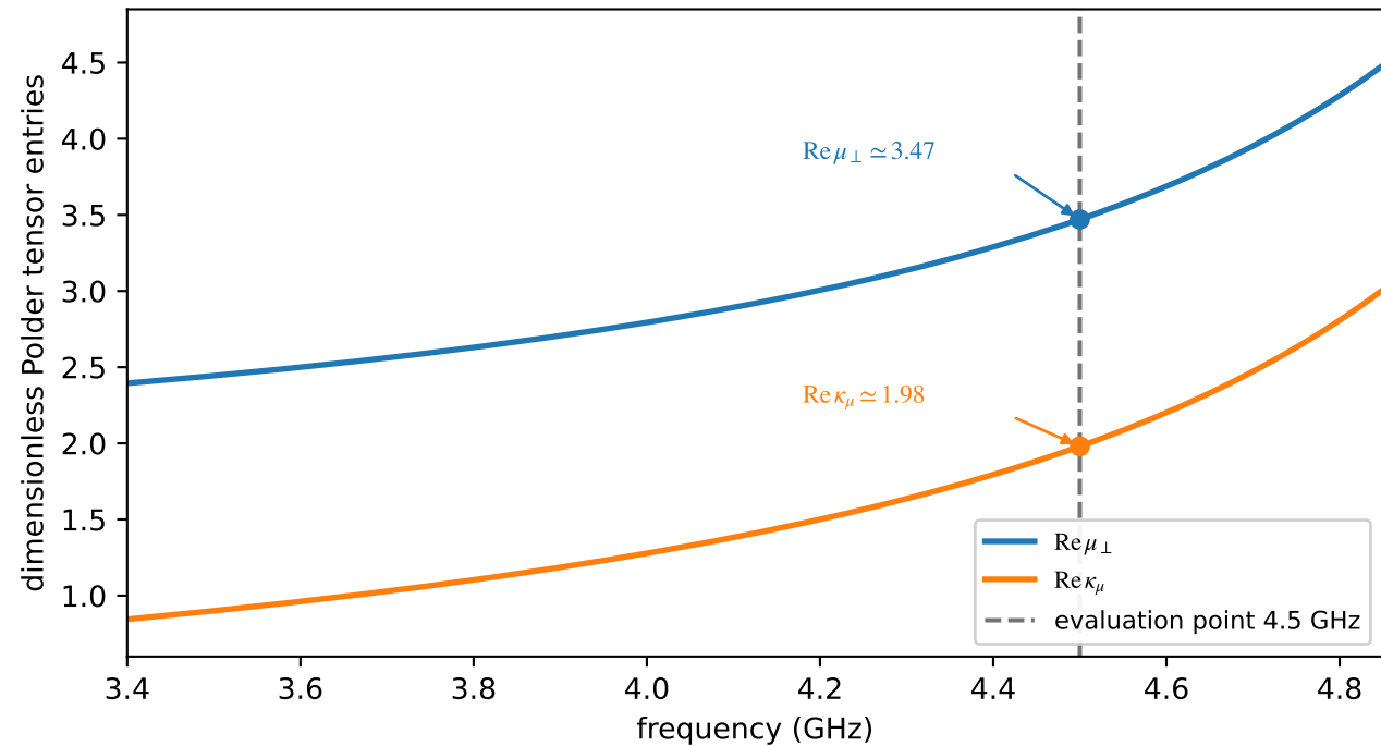
YIG Polder tensor components below resonance
