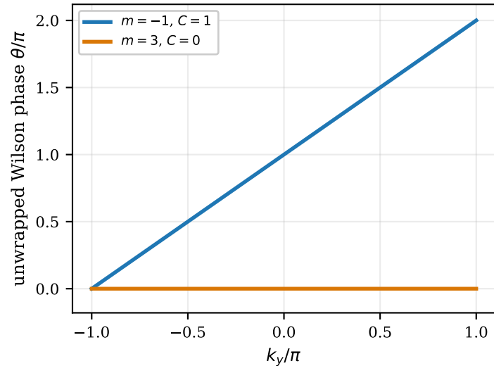
Wilson-loop winding
