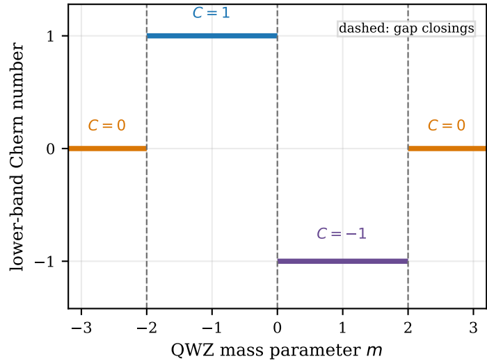
Chern plateaus vs mass
