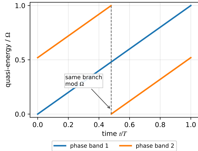
(a) phase bands modulo \Omega
