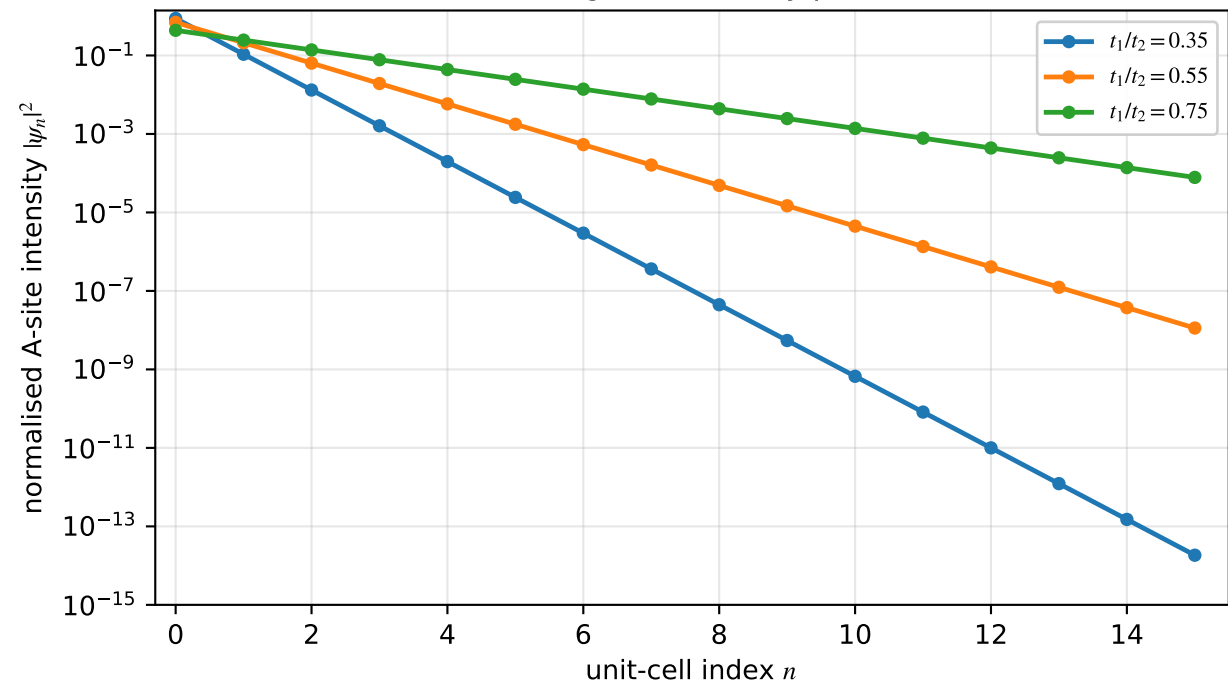
SSH edge-state decay profile
