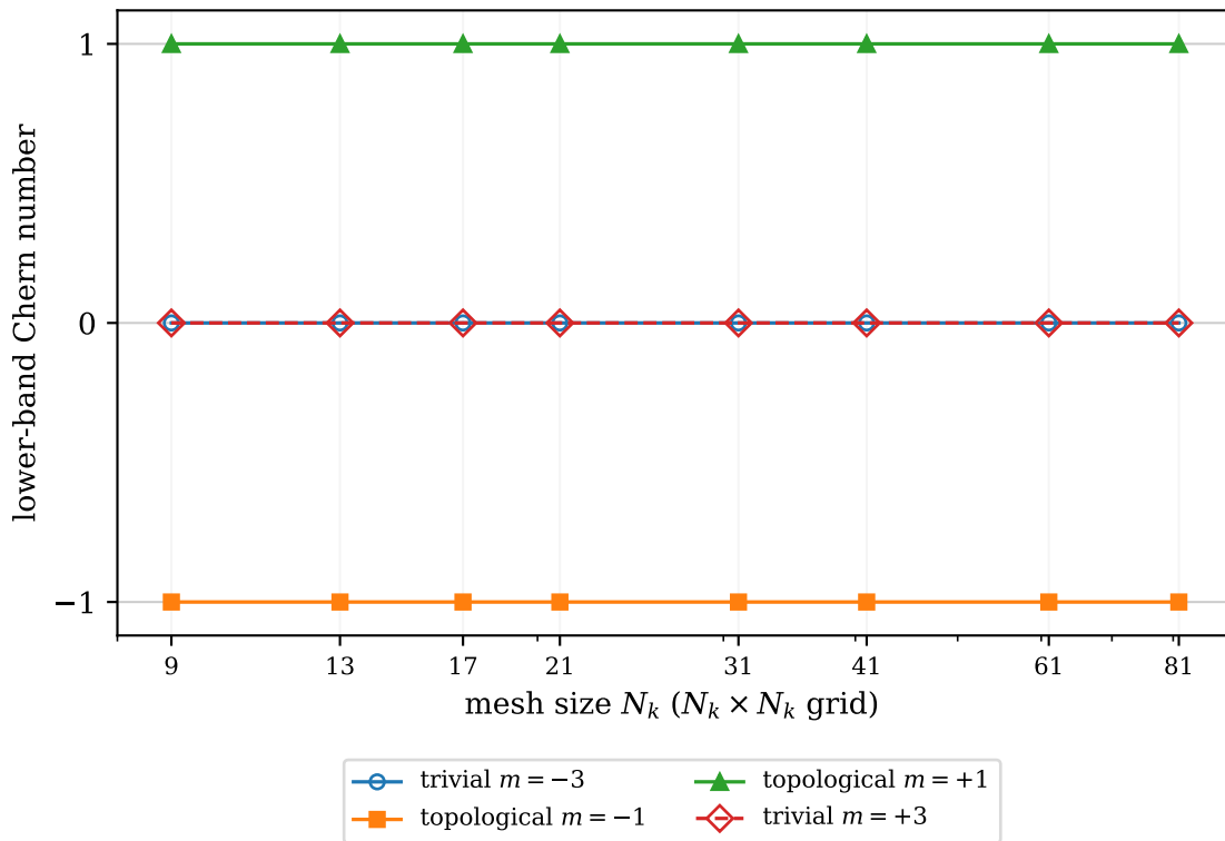
Plaquette Chern number for the QWZ model
