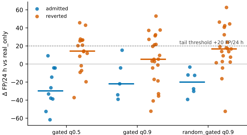
The gate's decision separates the false-alarm tail, within every arm
