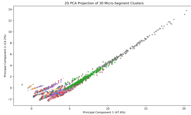
Figure 6: 2D PCA Cluster Projection. High-resolution projection of the 30 micro-segments, illustrating the dense behavioral and spatial variance captured by our model's peer grouping strategy.
