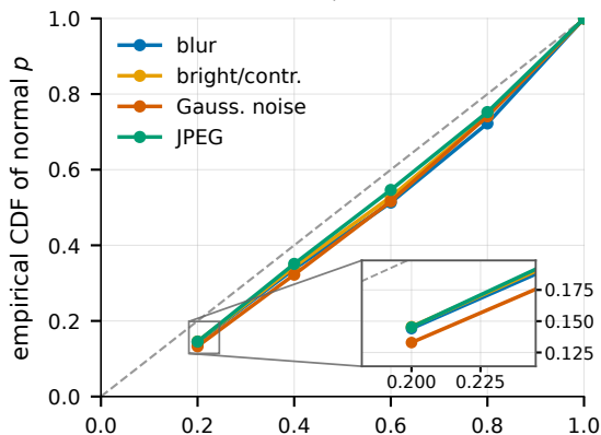
MVTec, k = 4
