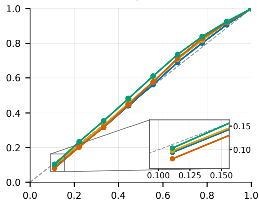
MVTec, k = 8
