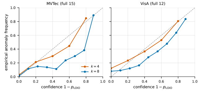
Figure 2: LOIO reliability diagrams on the full MVTEC (left) and VisA (right) corruption benchmarks, pooled over classes, seeds, and corruptions. Points occupy the k+1 attainable confidence levels; positions below the diagonal indicate overconfidence.
