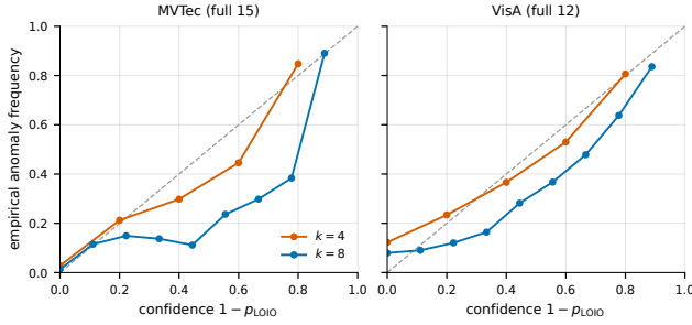
Figure 2: Reliability diagrams for LOIO conformal reliability on the full MVTec (left) and VisA (right) corruption benchmarks, pooled over classes, seeds, and corruptions. Points occupy the k+1 attainable confidence levels; gaps below the diagonal indicate overconfidence, which is larger at k=8 , consistent with the uniformity analysis in Section 5.5.
