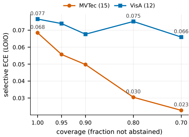
Figure 5: Overlaid risk-coverage curves for LOIO conformal reliability with entropy-ranked abstention on full MVTec and VisA. Abstaining on the 20% most uncertain images halves the remaining calibration error on MVTec.
