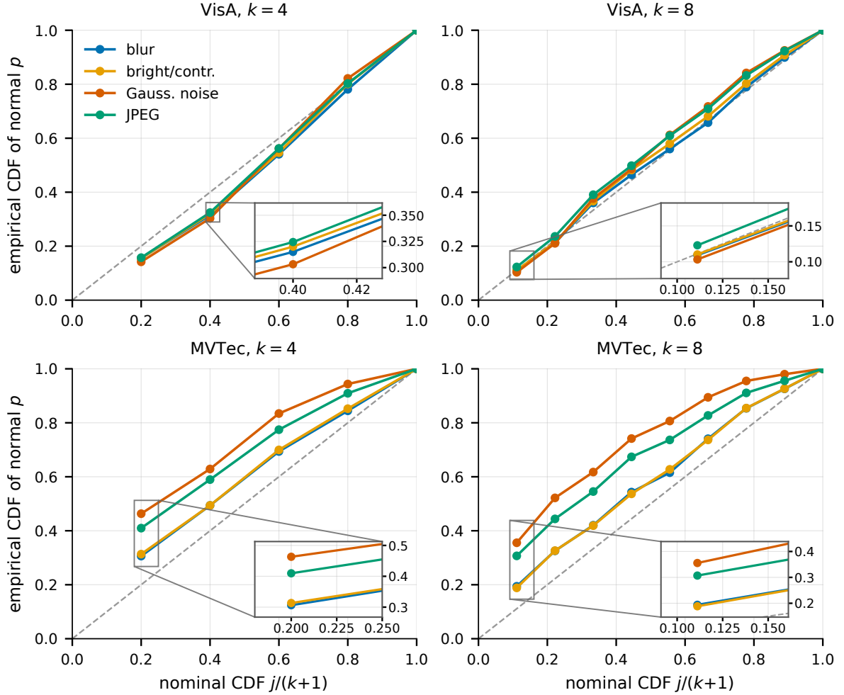
Figure 4: Discrete CDF comparison for normal-image LOIO p-values: empirical CDF at each attainable grid point j/(k+1) against the idealized exchangeable reference (dashed diagonal), per corruption. Points above the diagonal indicate excess false alarms relative to that reference. VisA k=4 is conservative; VisA k=8 and MVTec drift anti-conservative under corruption, worst for Gaussian noise. The lower-right insets enlarge the first informative grid region while occupying data-free areas of their parent panels.
