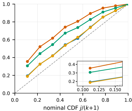
MVTec, k = 8
