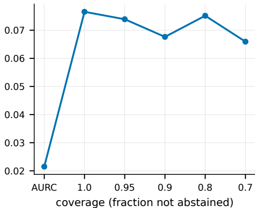
VisA (full 12)
