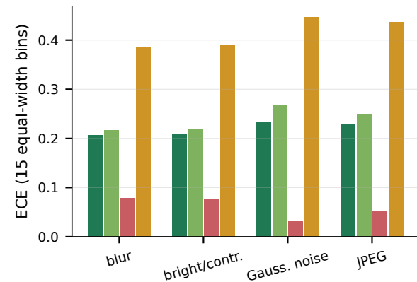
MVTec, k = 4
