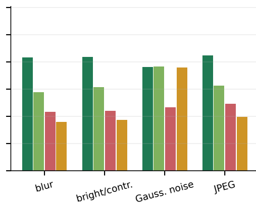
MVTec, k = 8
