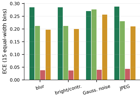
MVTec, k = 4
