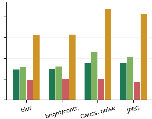
MVTec, k = 8
