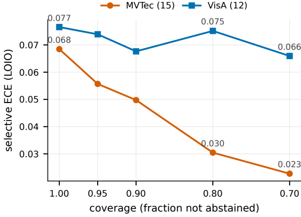
Figure 5: LOIO risk-versus-coverage curves with entropy-ranked abstention on full MVTec and VisA. Coverage is the retained image fraction; risk is ECE on the retained subset.
