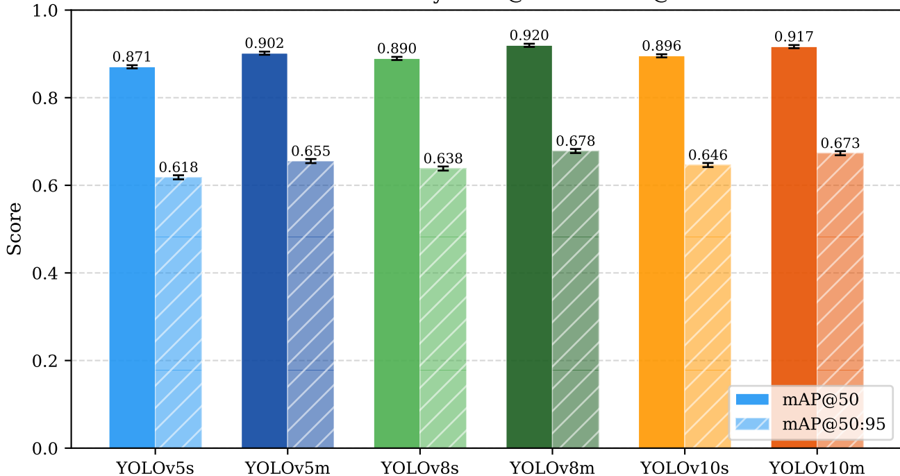
Detection Accuracy: mAP@50 and mAP@50:95
