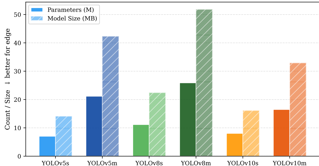
Model Efficiency: Parameters vs. File Size
