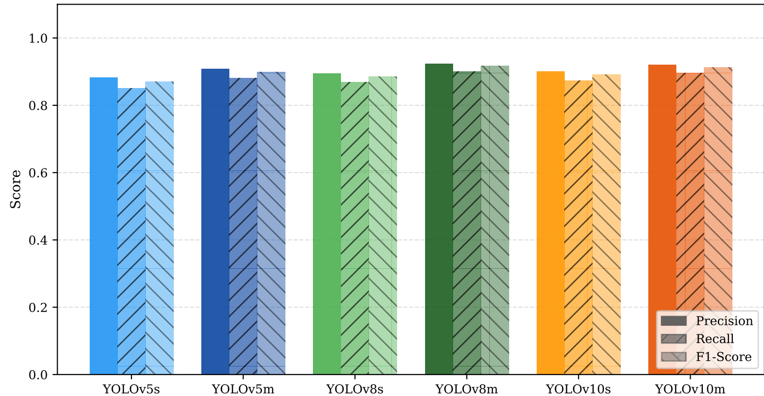
Precision, Recall, and F1-Score per Model
