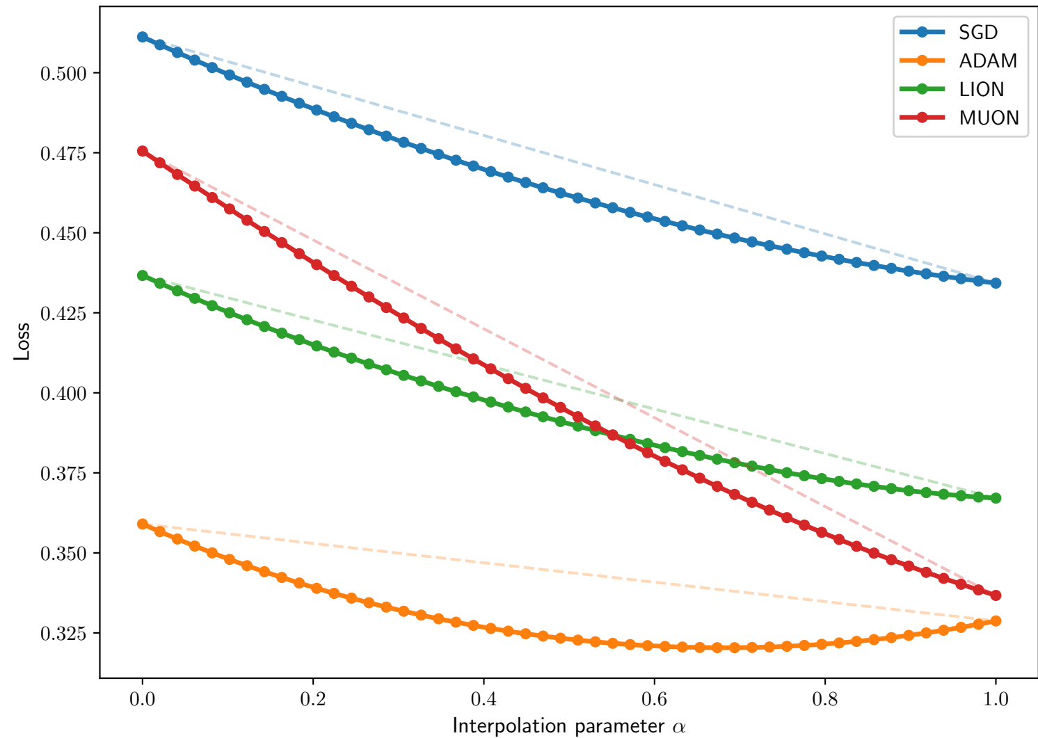
Loss Trajectories — Epoch 2
