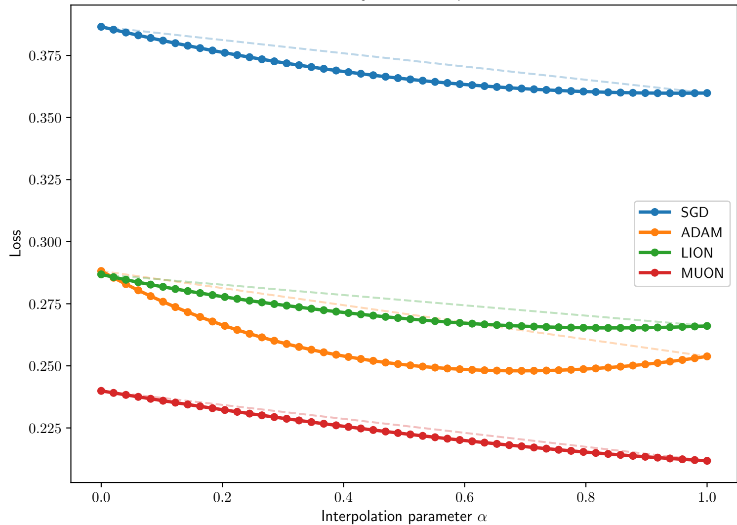
Loss Trajectories — Epoch 5
