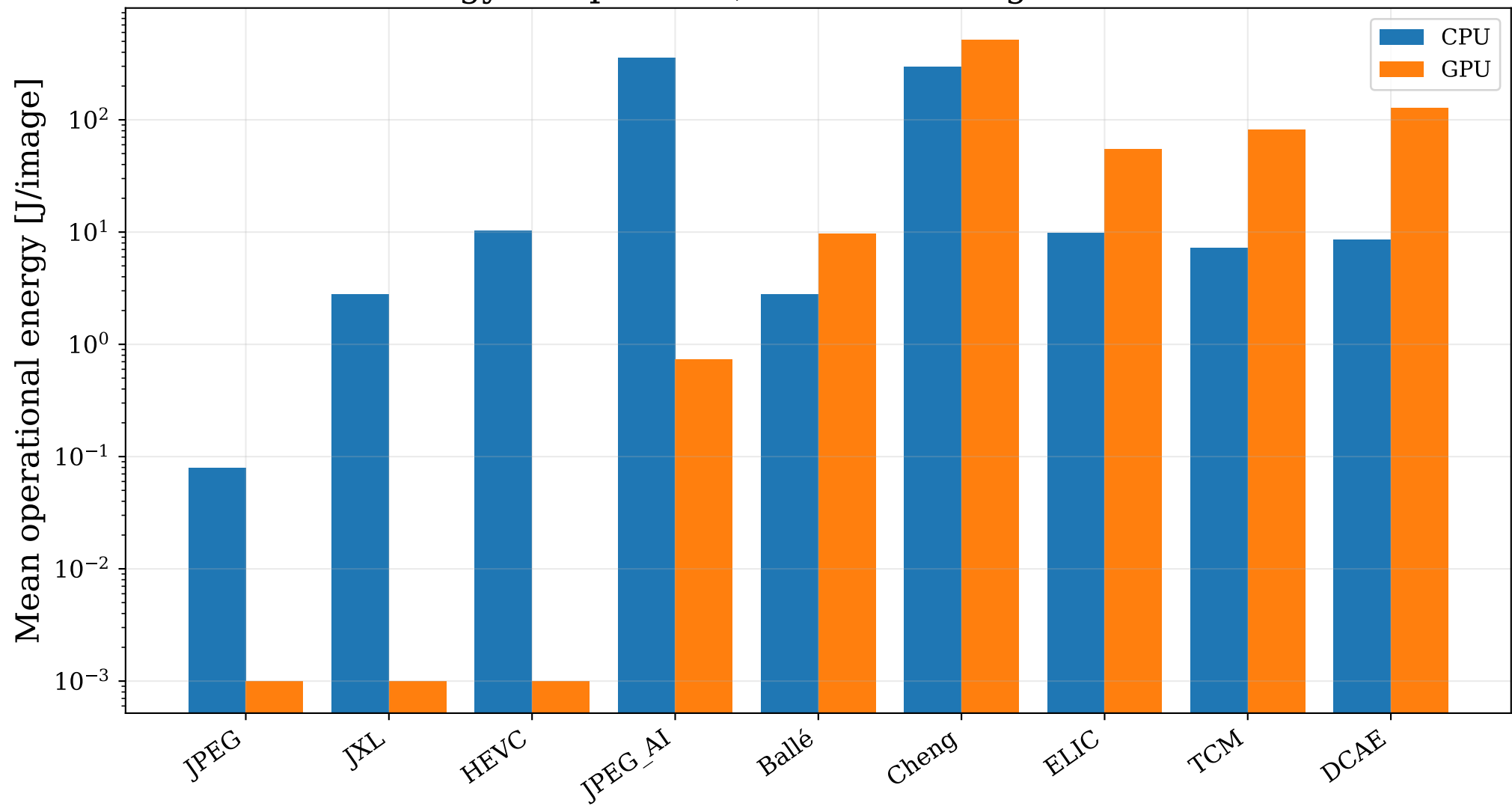
Energy components, 4-dataset image benchmark
