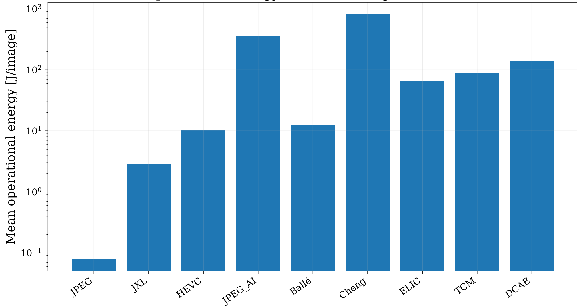
Operational energy, 4-dataset image benchmark
