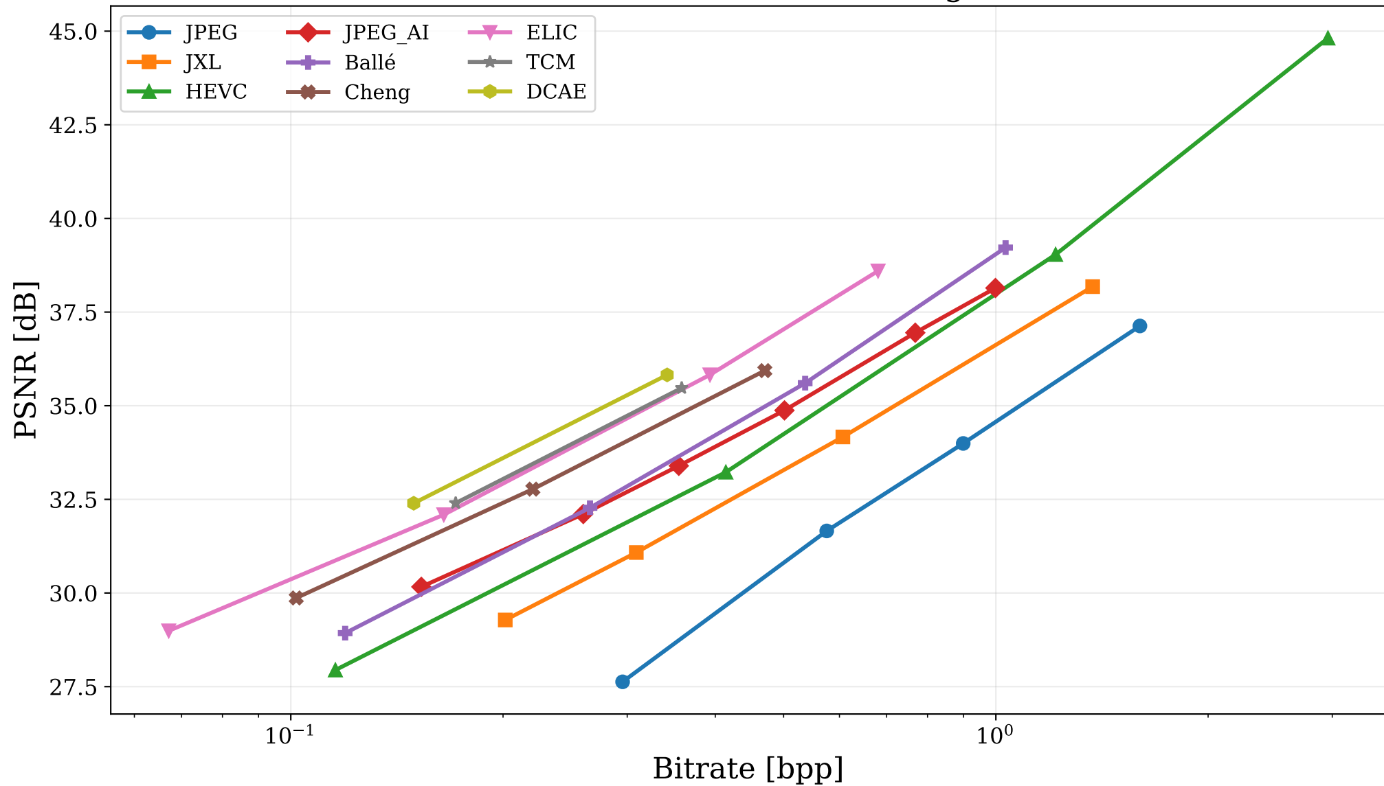
Rate-distortion, PSNR, 4-dataset image benchmark
