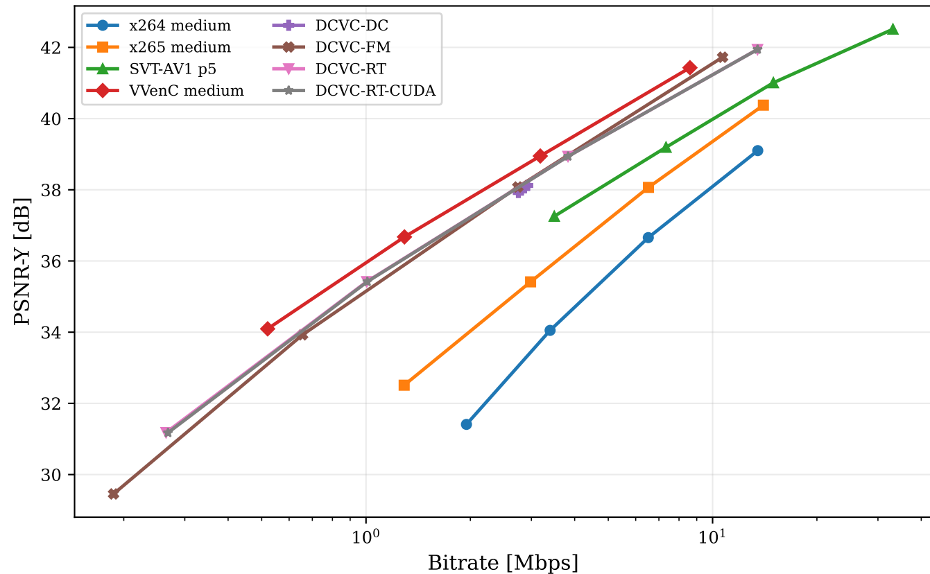
Rate-distortion, PSNR-Y, LDP reference presets
