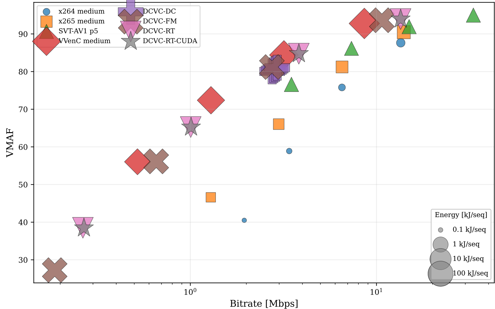
Rate--distortion--energy operating space
