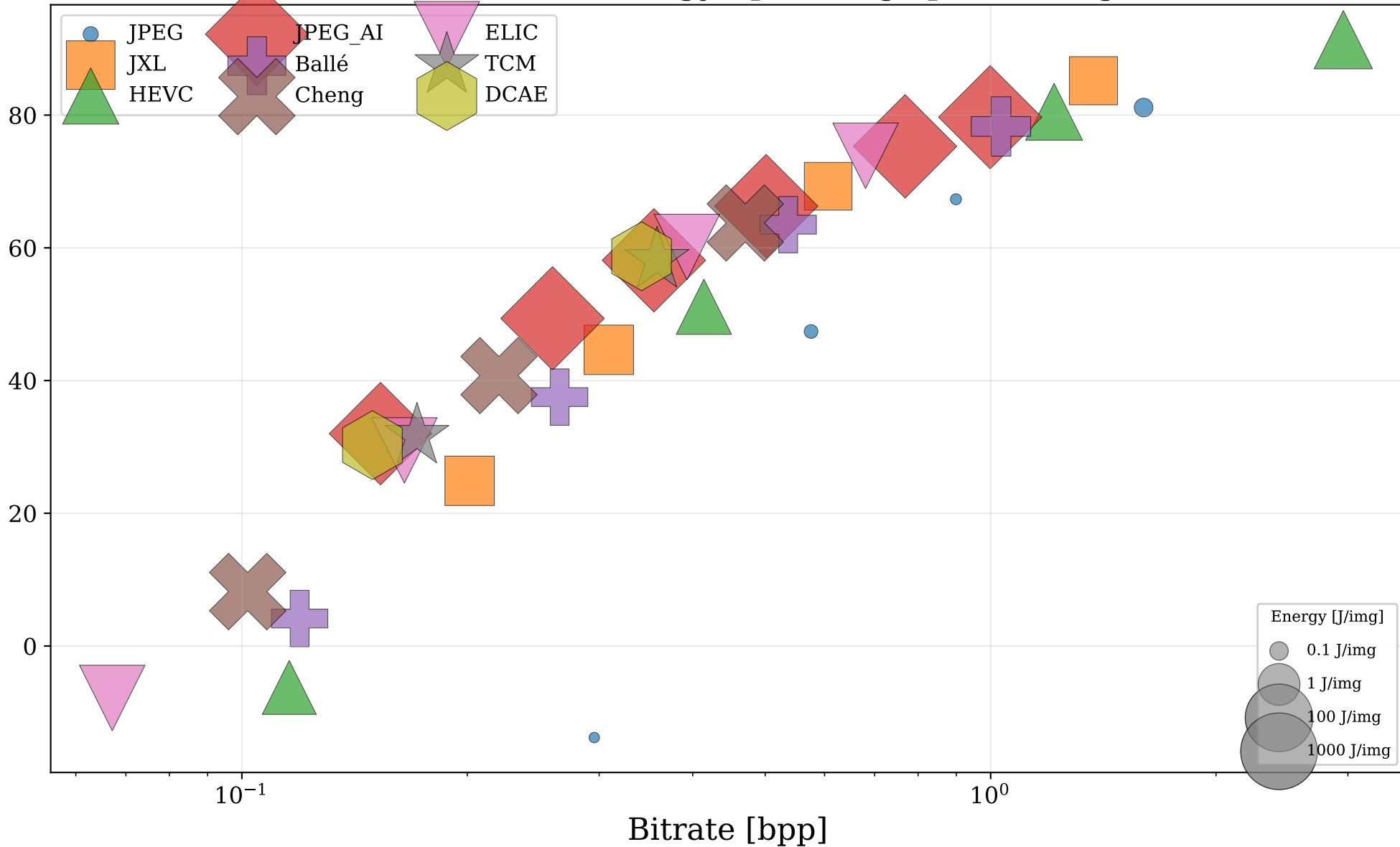
Rate--distortion--energy operating space, images
