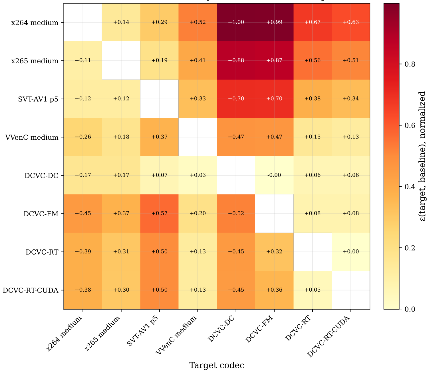
Additive \varepsilon -indicator heatmap, R-D-E, LDP reference presets
