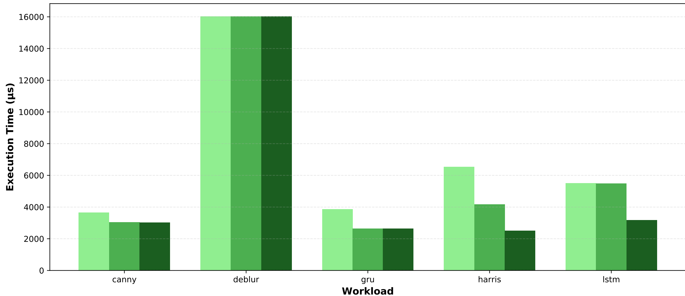
SoC Resource Scaling Comparison - GEDF_D
