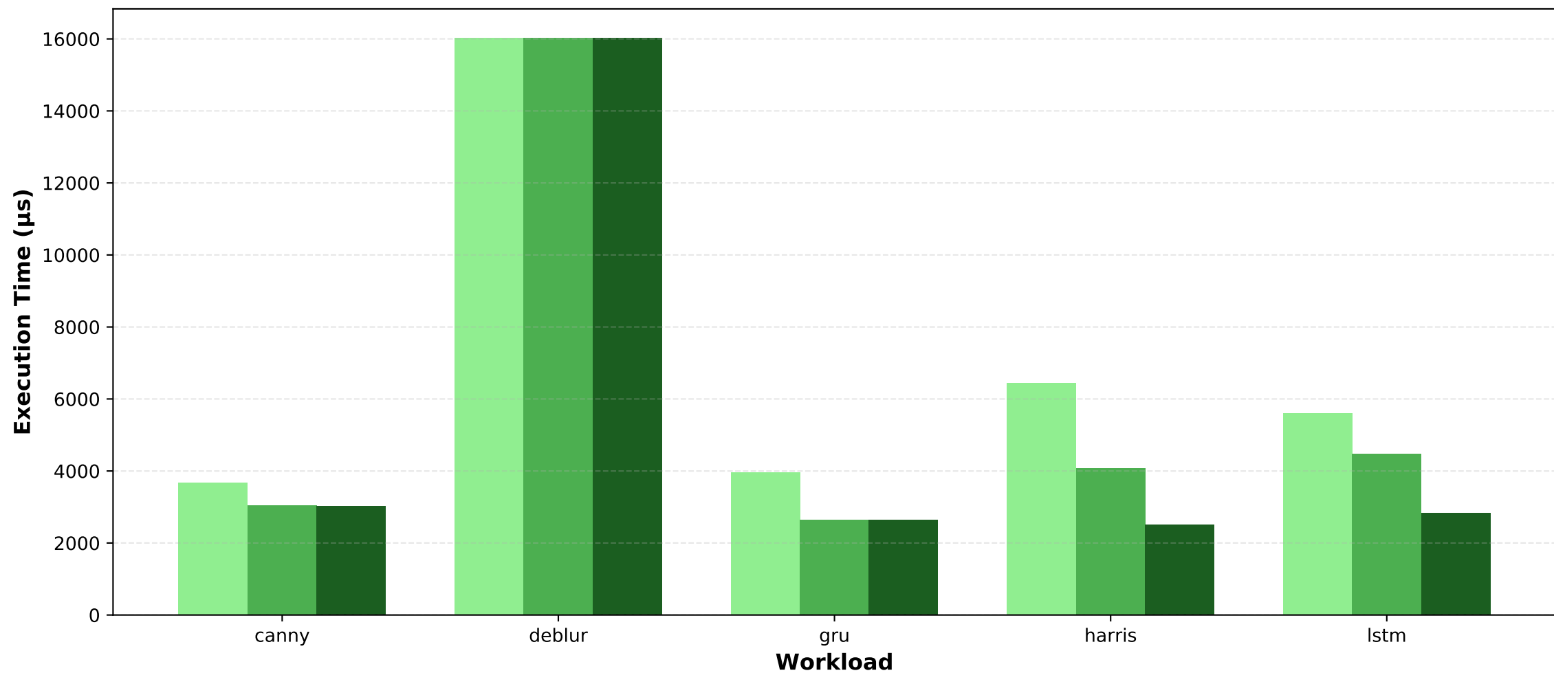
SoC Resource Scaling Comparison - GEDF_N
