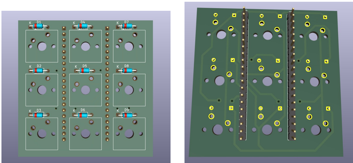
(a) Vista 3D Superior (Diodos e Soquetes MX).
