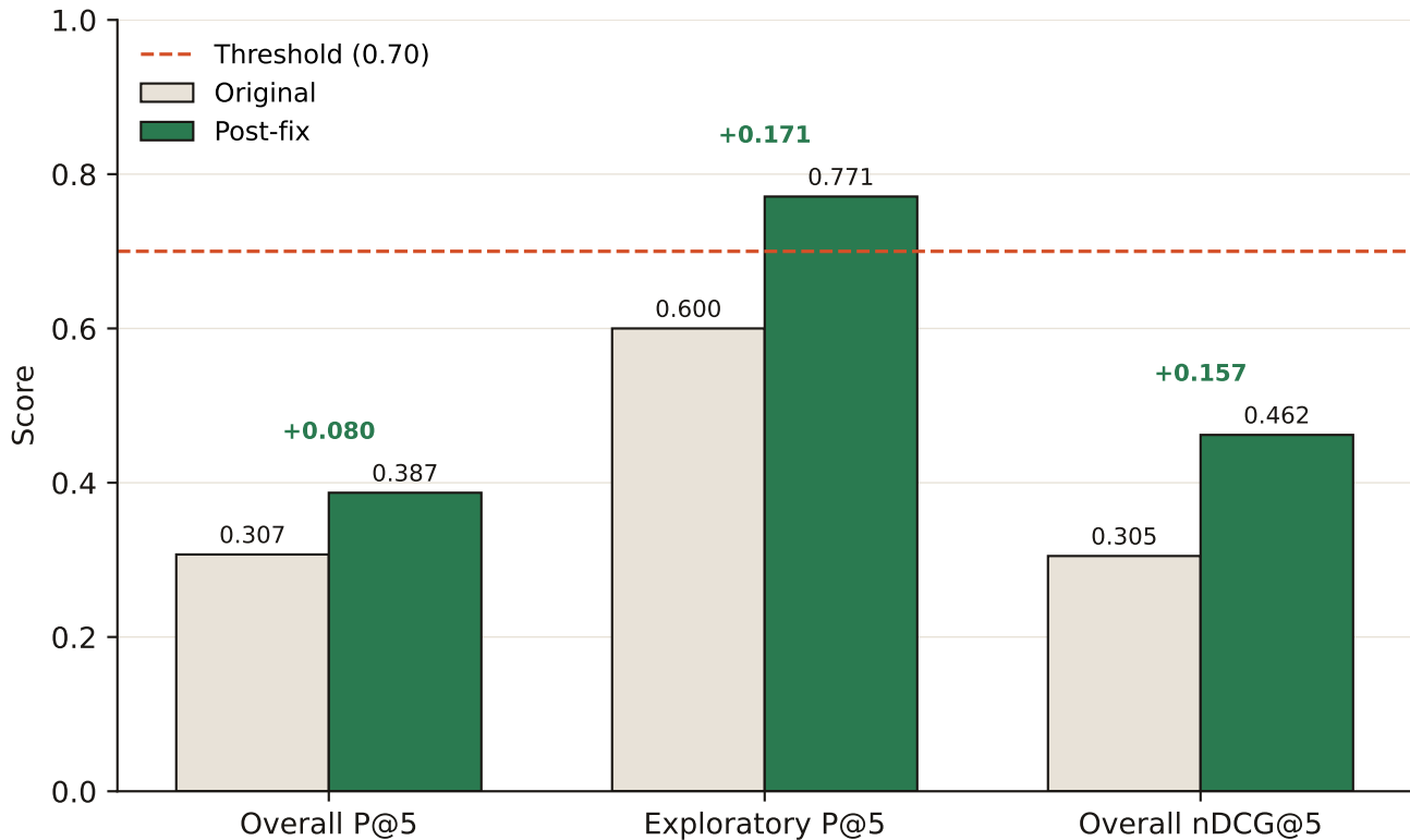
VOYO Retrieval Quality — Original vs Post-Fix Rerun
