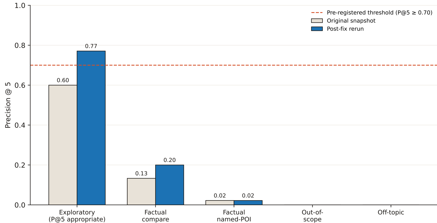
Retrieval P@5 by Query Pathway — Original vs Post-Fix
