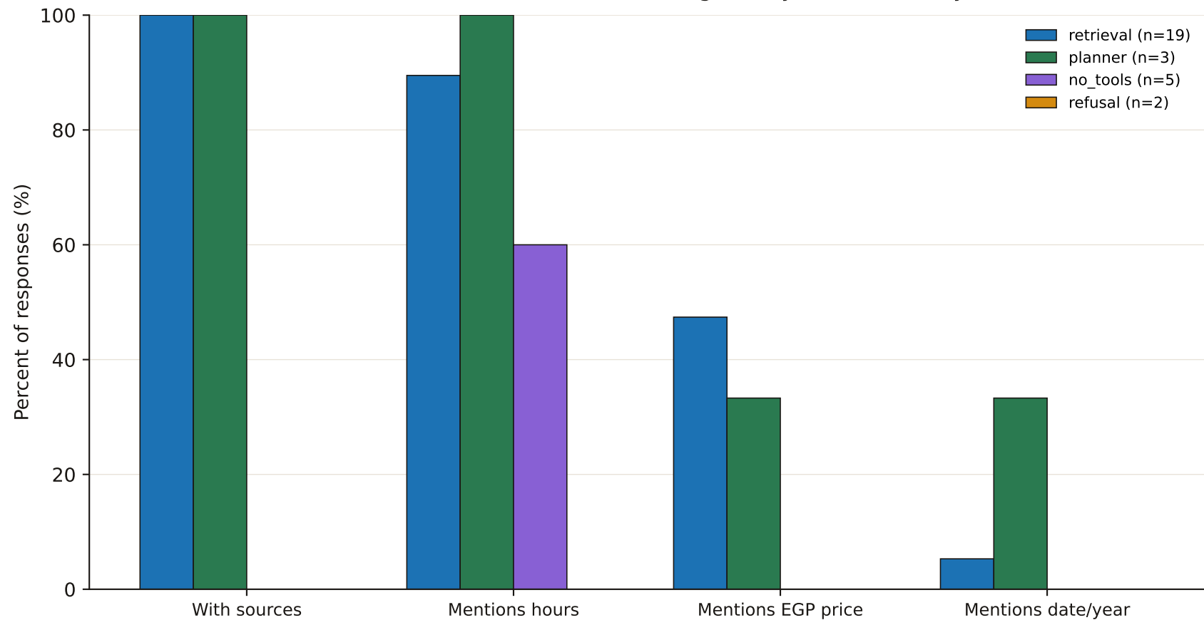
Conversational Groundedness Signals by CLEO Pathway
