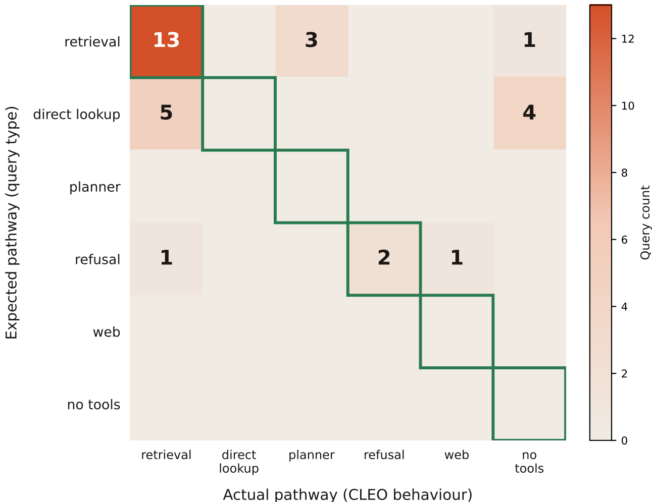
CLEO ReAct Routing — Confusion Matrix Overall routing accuracy: 50.0% (n=30, post-fix)
