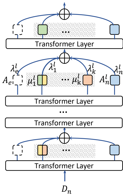
Architecture Search Procedure
