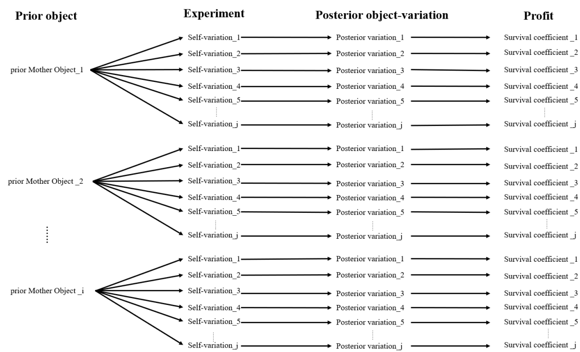
Figure 5.purpose-based Survival Tensor
