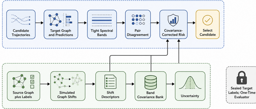
Figure 1: SPECTRA-DA pipeline. Frozen candidate predictions are decomposed over a tight target-graph spectral frame. Observable band-wise disagreement is combined with error covariance transported from labeled source simulations, yielding covariance-corrected target-risk estimates without exposing target labels to the selector. The hidden labels are used only by the isolated evaluator after the selector is frozen.
