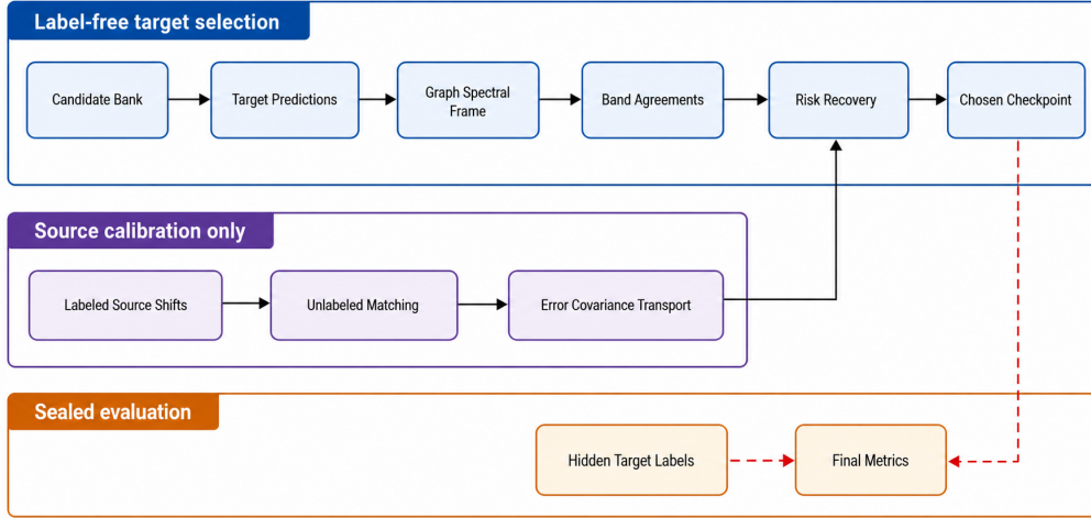
Figure 1: GDA-Select protocol and Spectra-DA research module. The selector sees a frozen candidate bank and unlabeled target predictions. Spectra-DA combines graph-spectral disagreement with covariance estimated from labeled source simulations. Target labels remain isolated in the evaluator. Under the registered audit reported in this paper, no selector passed all promotion guards, so the final twelve sealed transfers were not queried.
