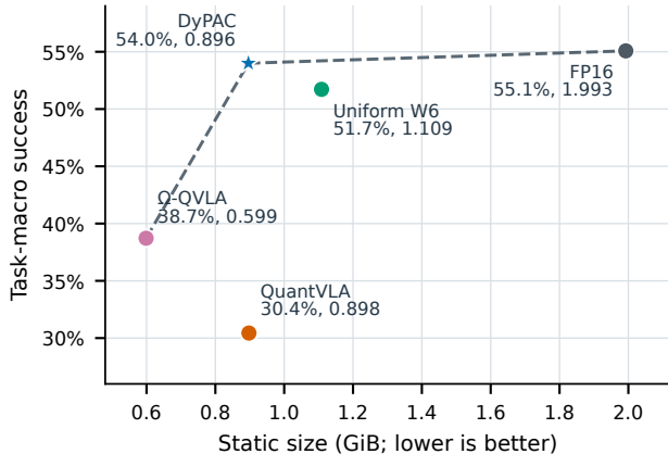
a GR00T success-storage
