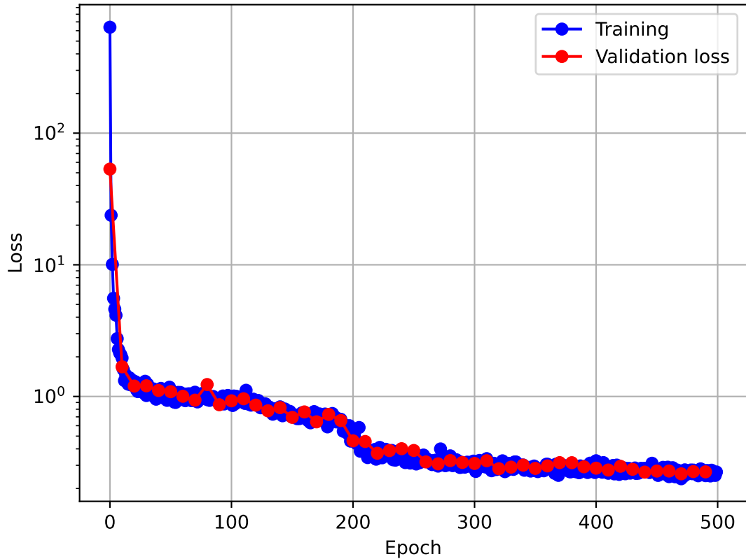
Training and Validation Loss Curves for N=10 , d=3 , \beta=2.82843 , a=1.0
