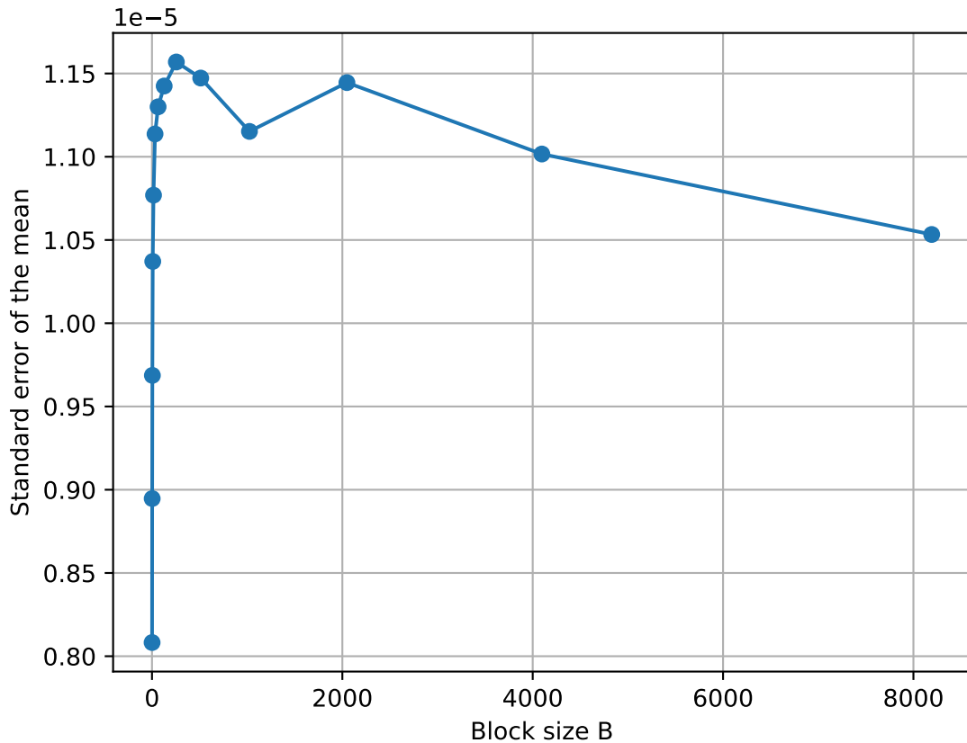
Standard error of the mean vs block size for N=2 , \beta=2.82843 , a=0.0
