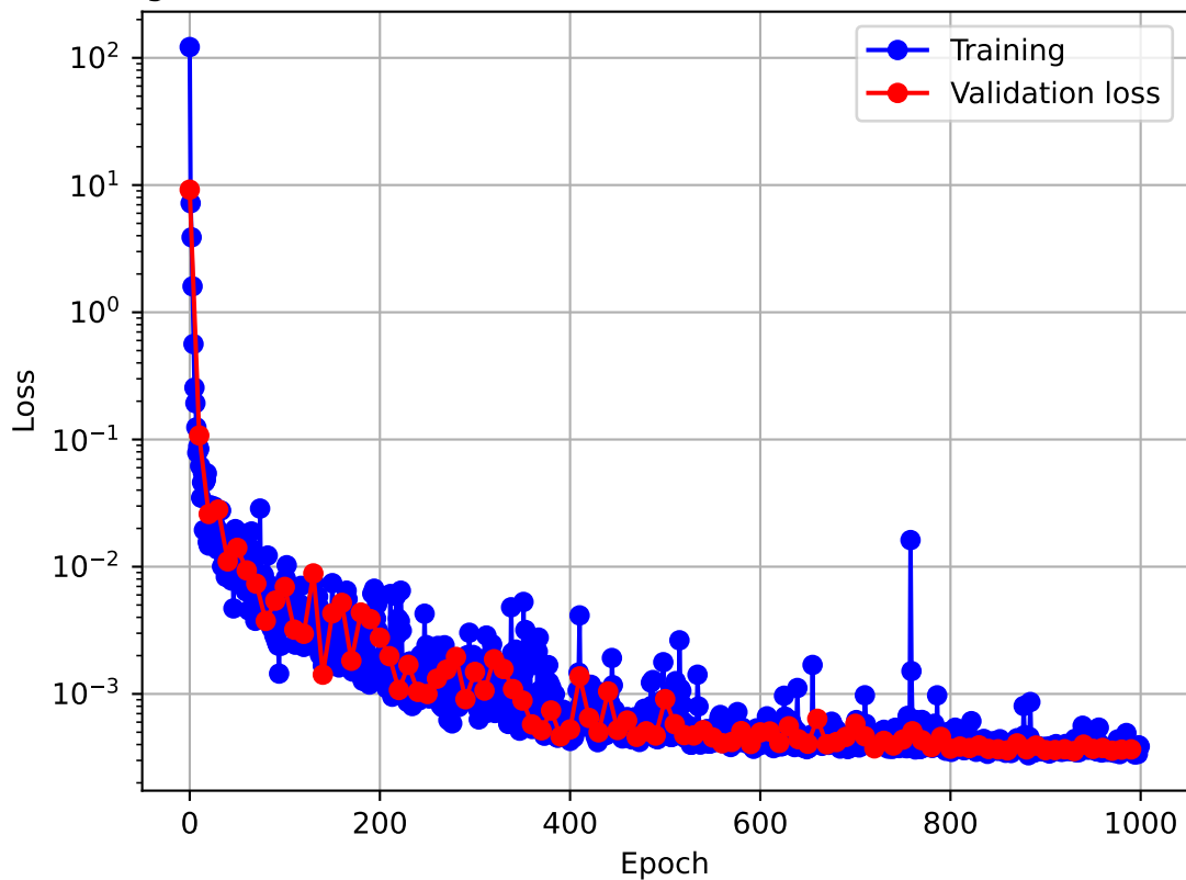
Training and Validation Loss Curves for N=2 , d=3 , \beta=2.82843 , \alpha=1.0
