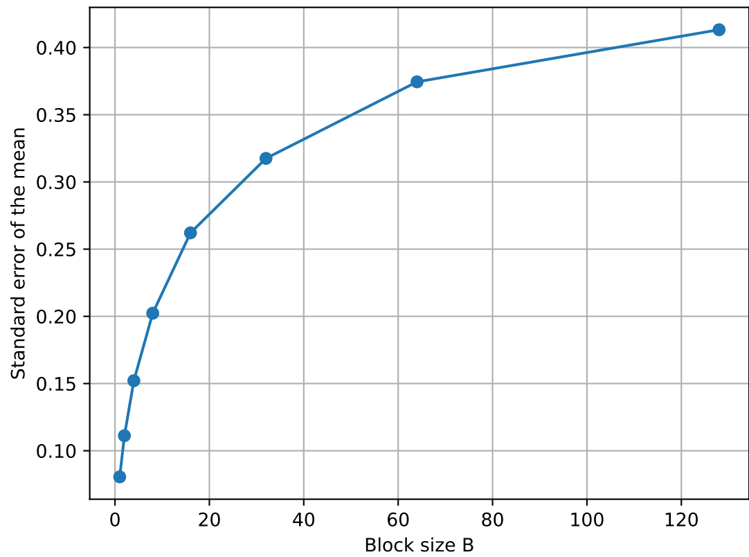
Standard error of the mean vs block size for N=10, beta=2.82843, a=0.004
