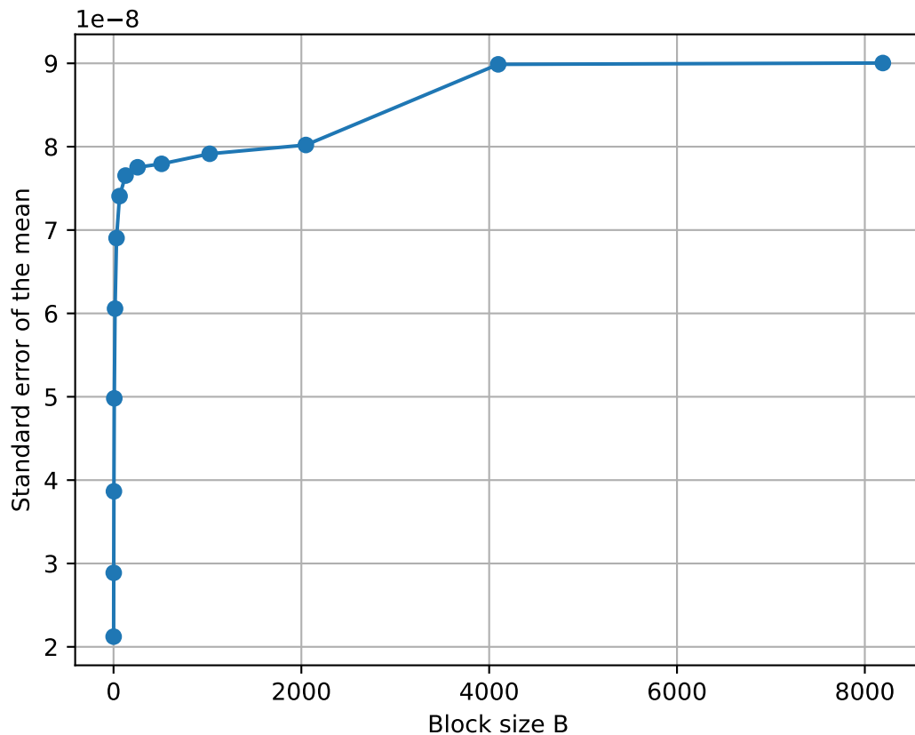
Standard error of the mean vs block size for N=10 , \beta=1.0 , a=0.0
