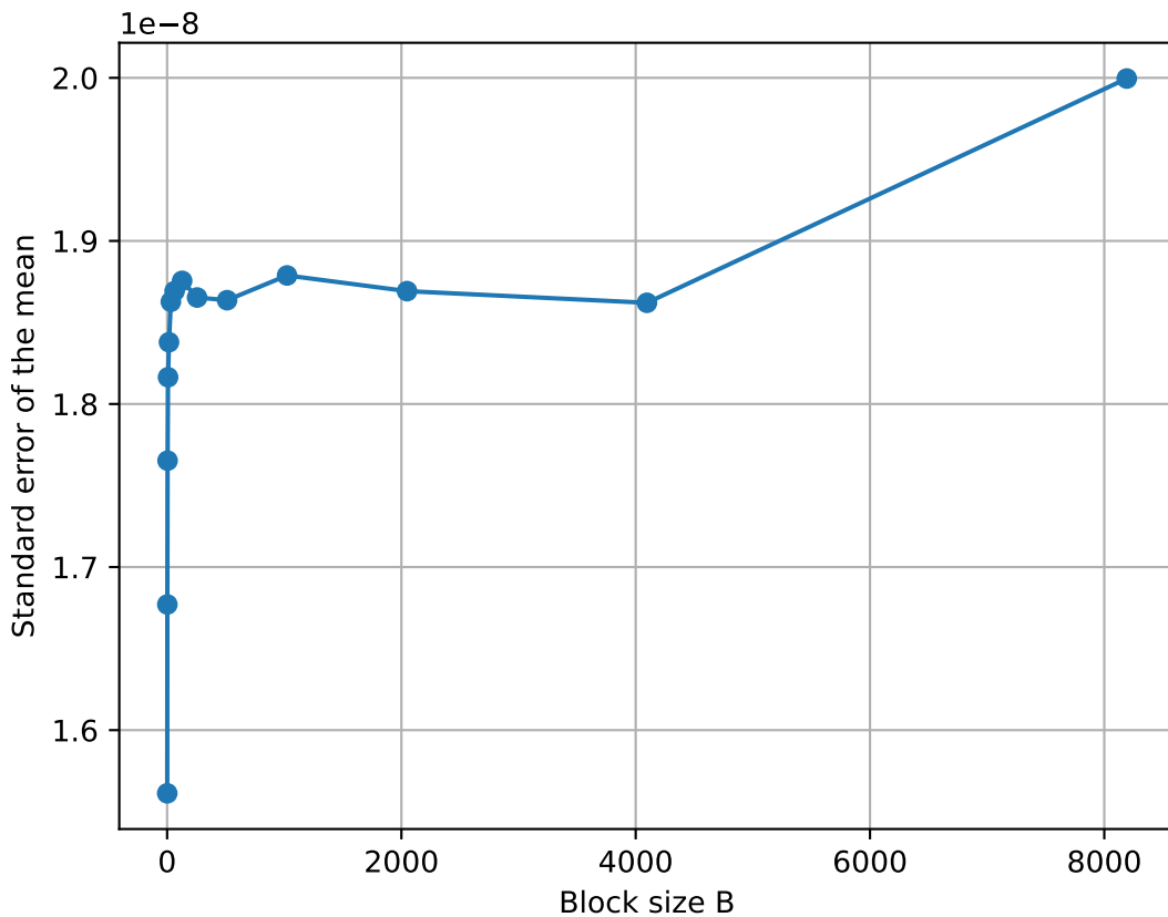
Standard error of the mean vs block size for N=1 , \beta=1.0 , a=0.0
