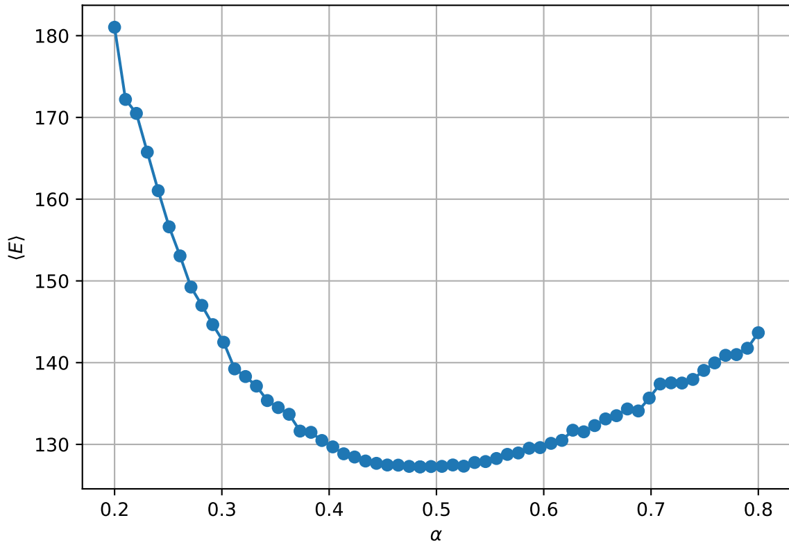
Interacting case: N = 50 , D = 3
